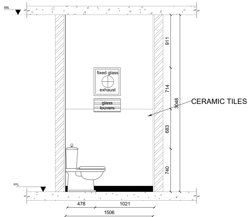
SECTIONAL ELEVATION
