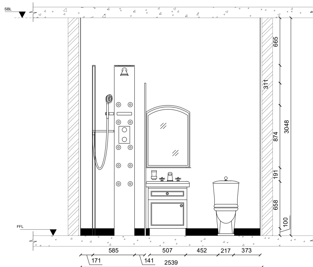
SECTIONAL ELEVATION
