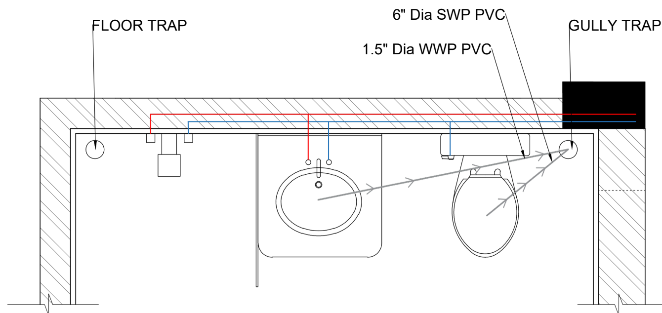
PLUMBING
