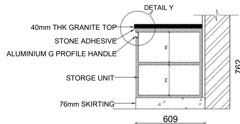
DETAIL X
