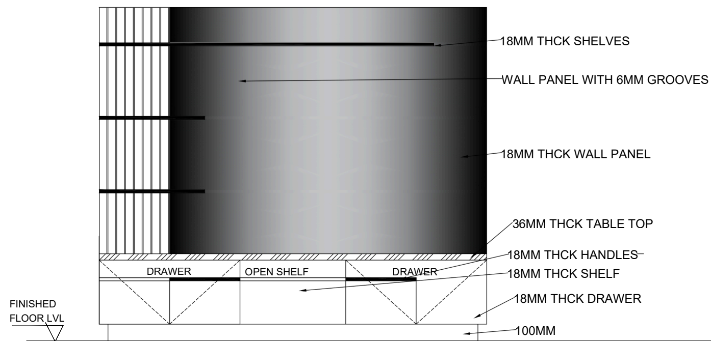
FRONT ELEVATION
