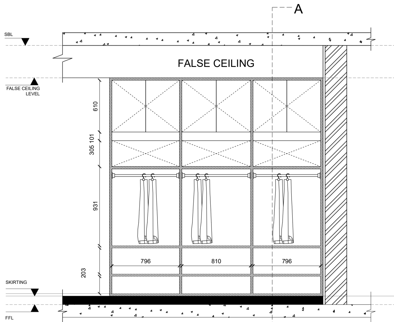
SECTIONAL ELEVATION
