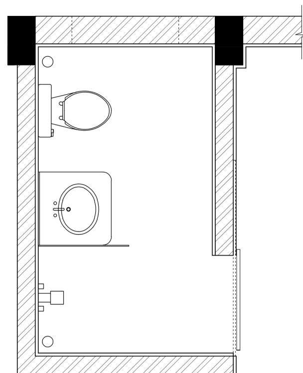
PLAN
